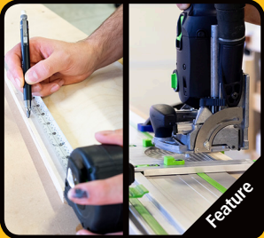
Layout mortise spots & attach Sled
