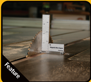
Set blade height safely
