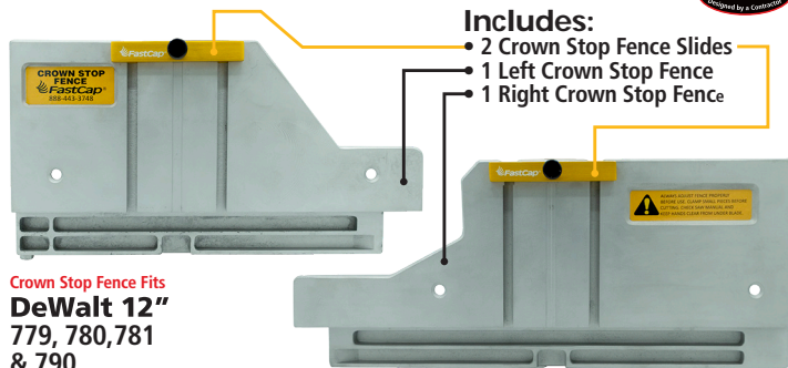
T-groove design & built in storage
