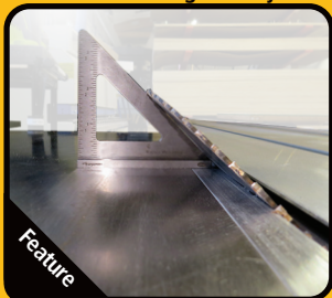
Set blade angle safely
