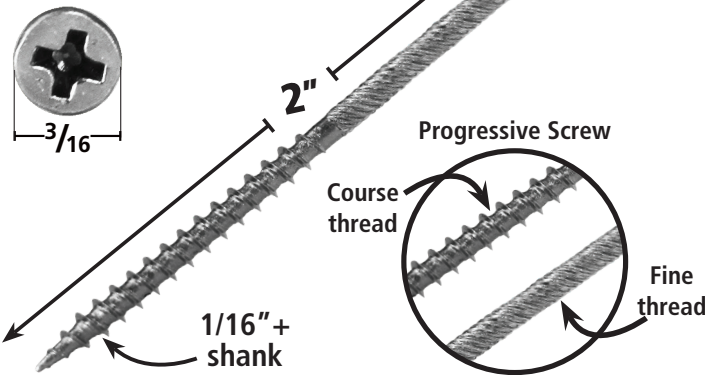
Large screws harder to cover up
