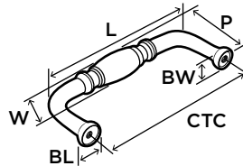
4 55243 96mm CTC
