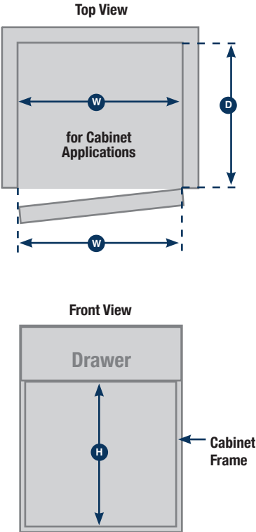
Example of Frameless / Euro-Style Cabinet and Door Application
