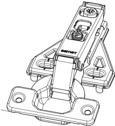
Features: KVSHB FD 501
